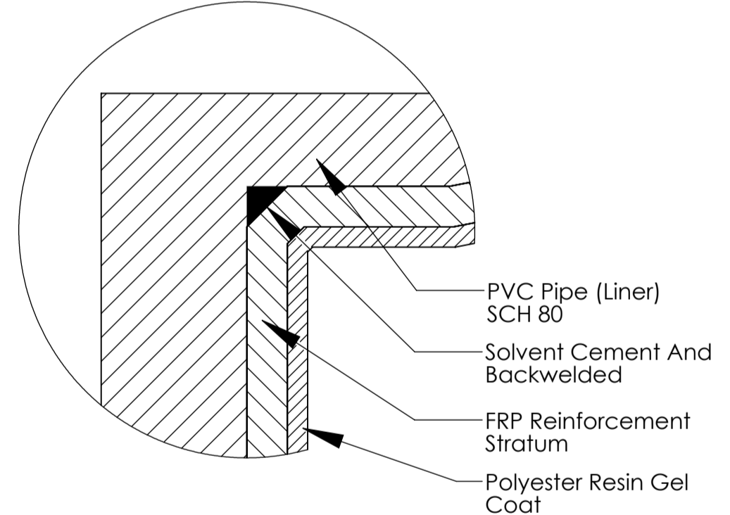
DETAIL A SCALE 1.5 : 1
